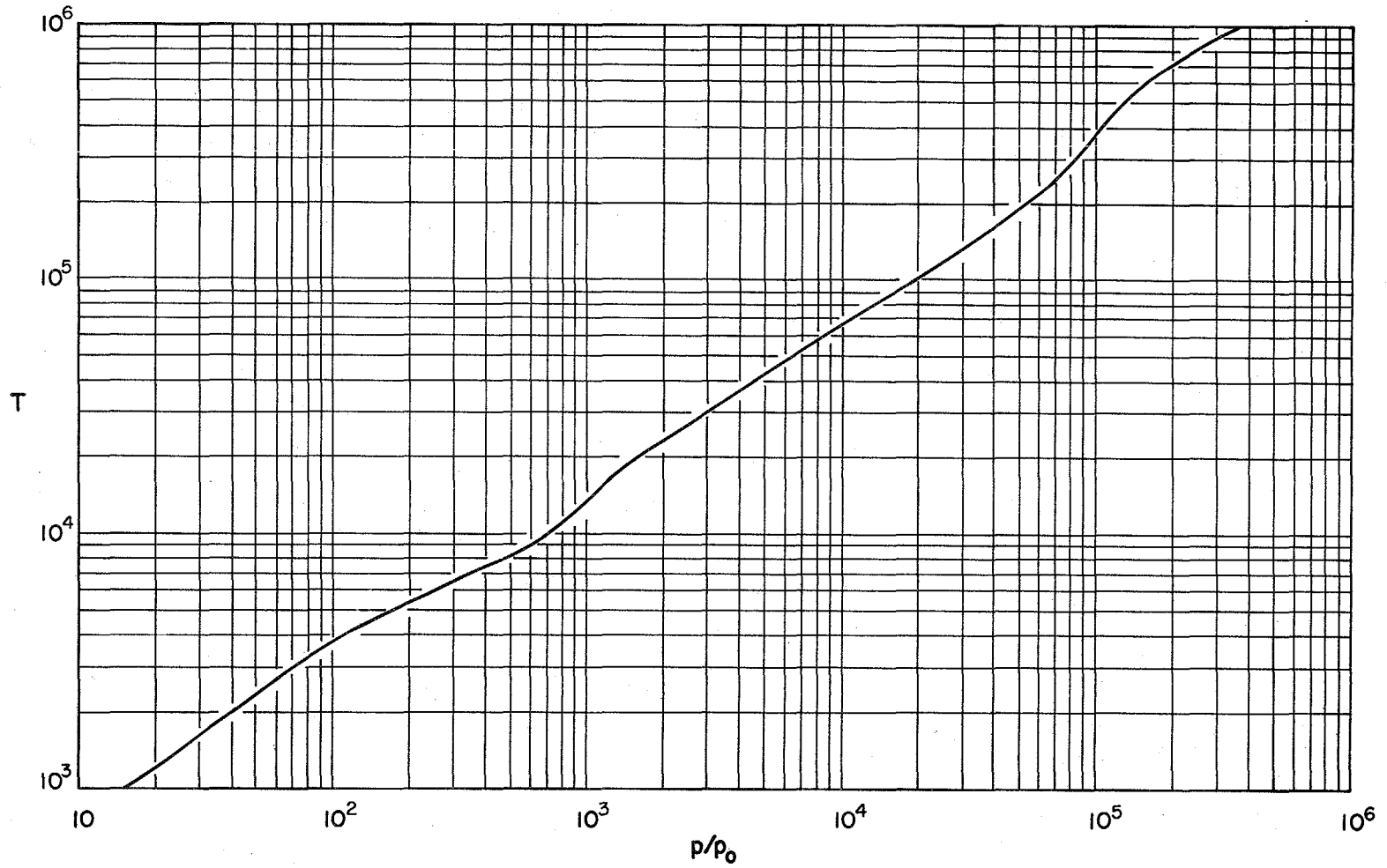
Fig. 7.3 Hugoniot curve; temperature as a function of shock pressure
