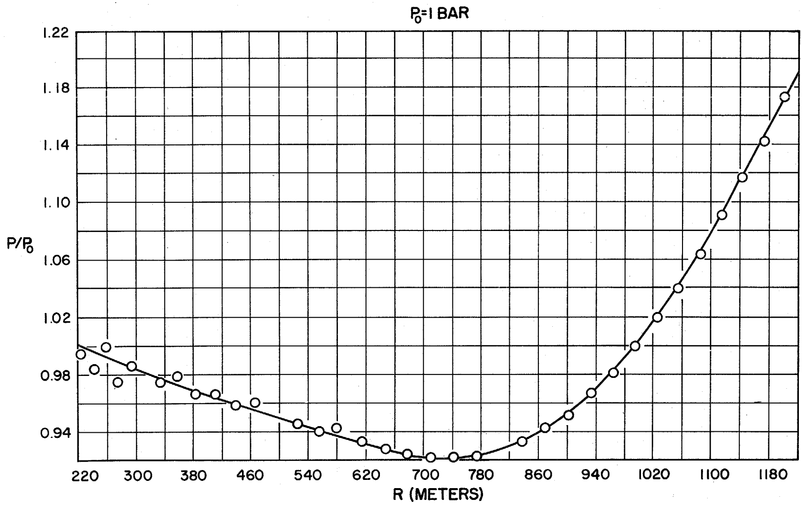
Fig. 6.10 Pressure vs distance at a fixed time
