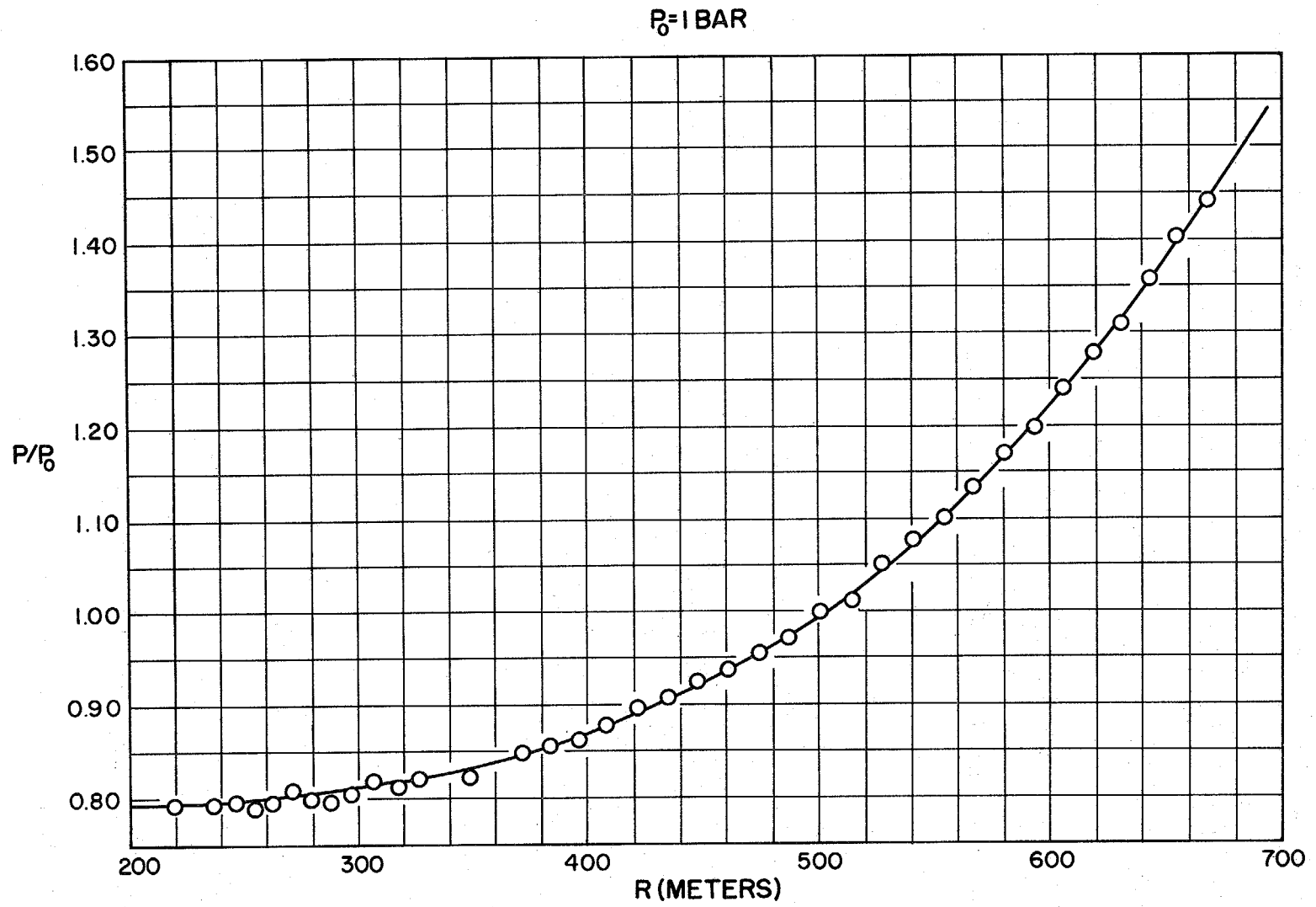
Fig. 6.9 Pressure vs distance at a fixed time
