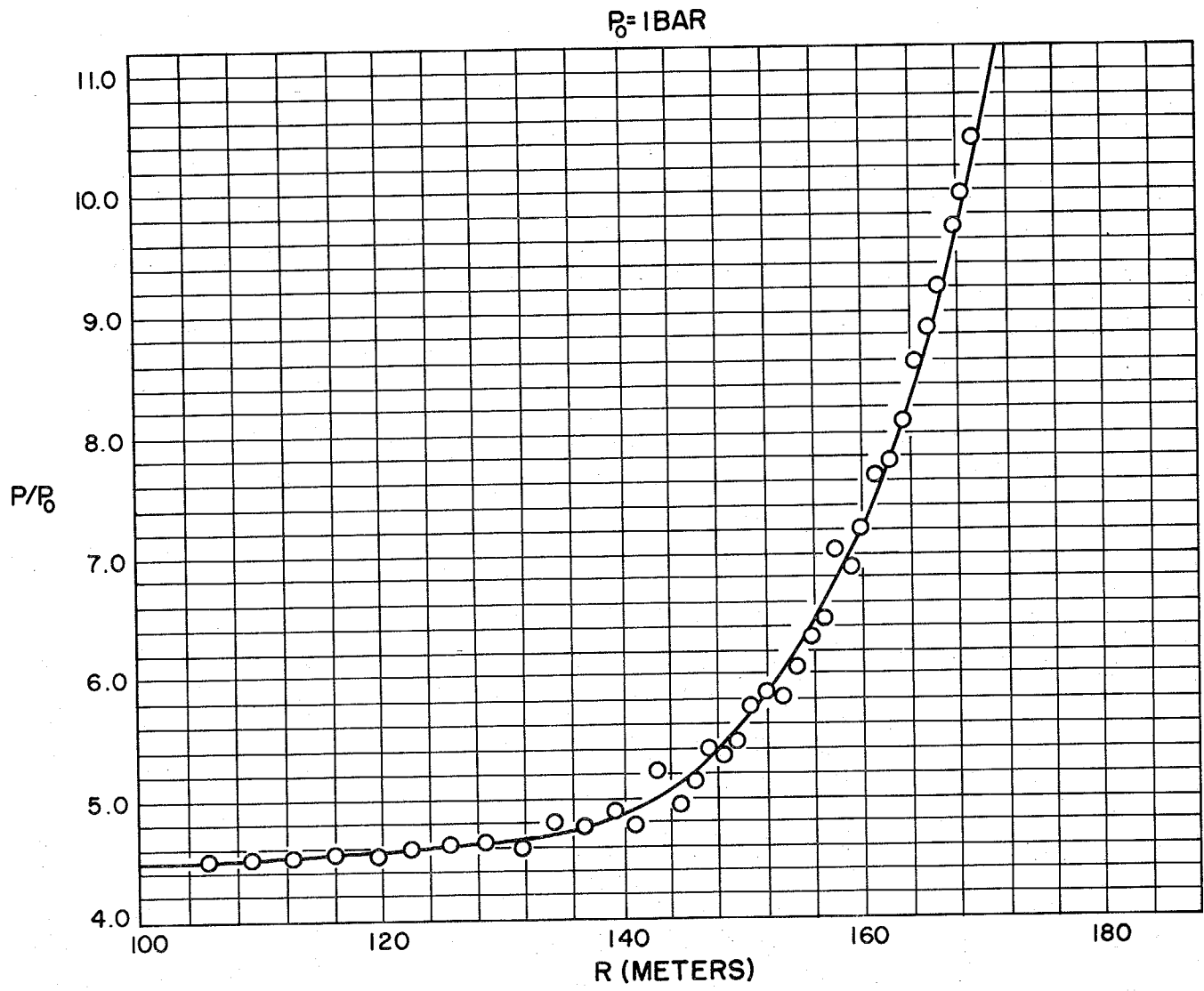
Fig. 6.5 Pressure vs distance at a fixed time
