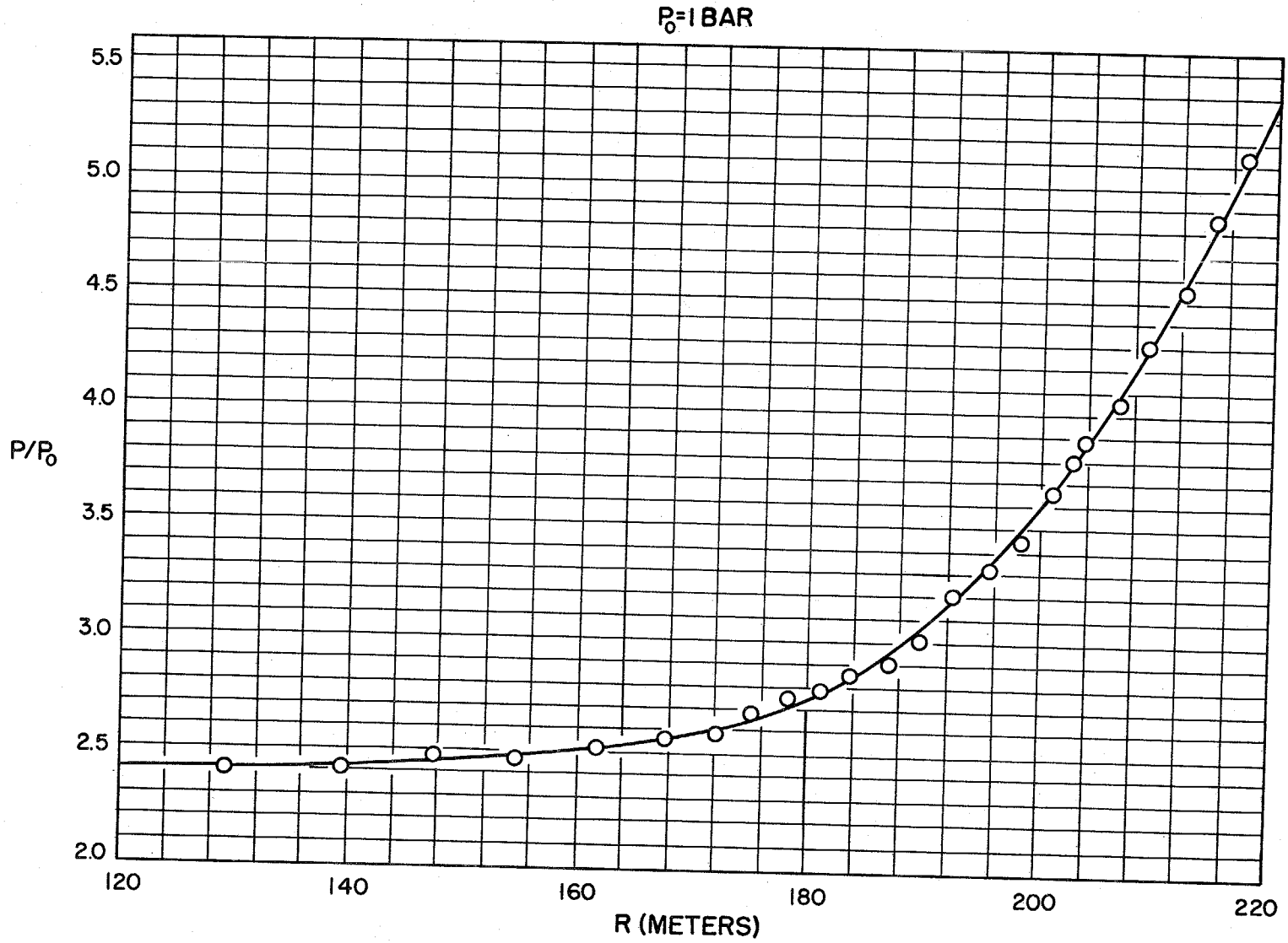
Fig. 6.6 Pressure vs distance at a fixed time
