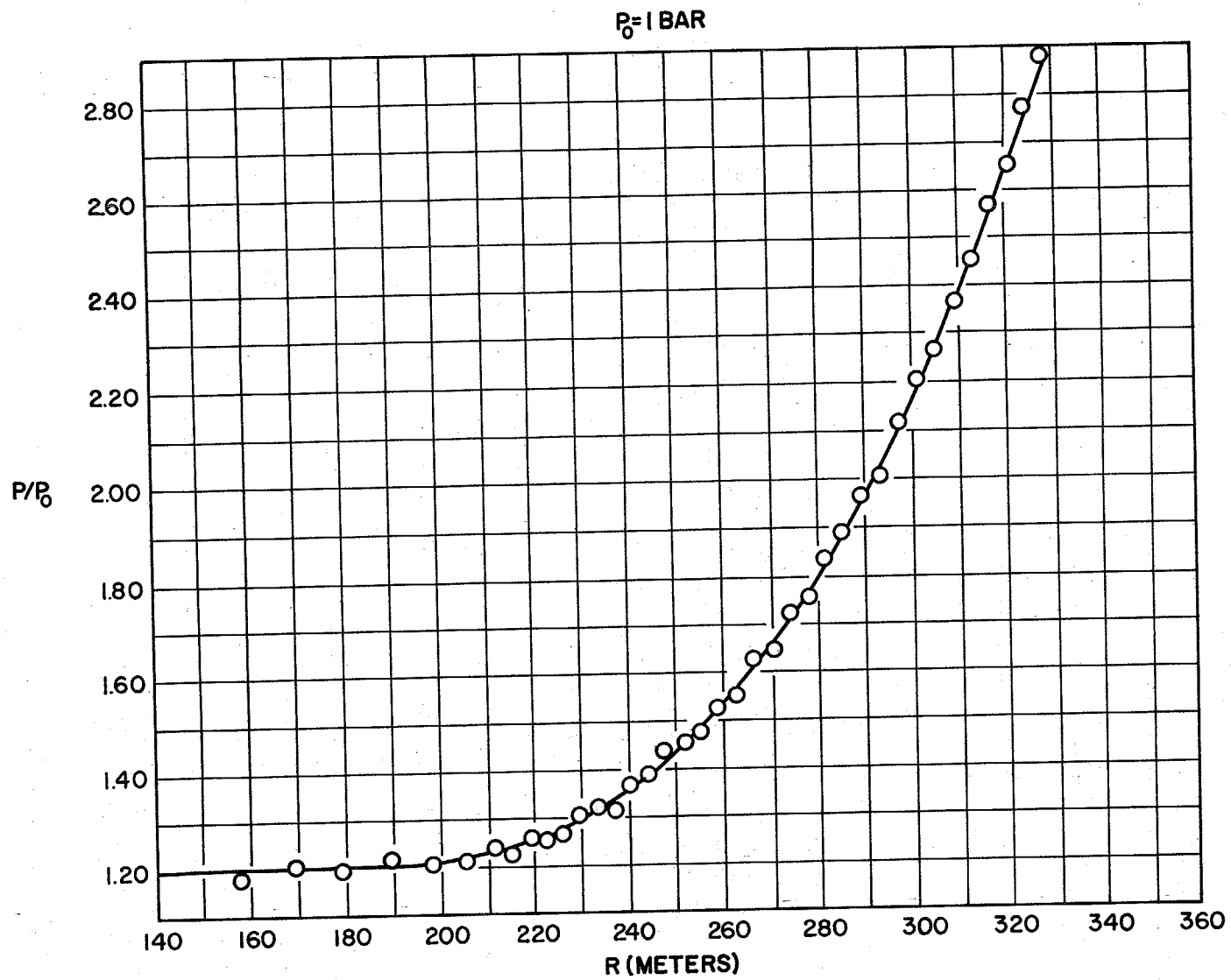
Fig. 6.7 Pressure vs distance at a fixed time
