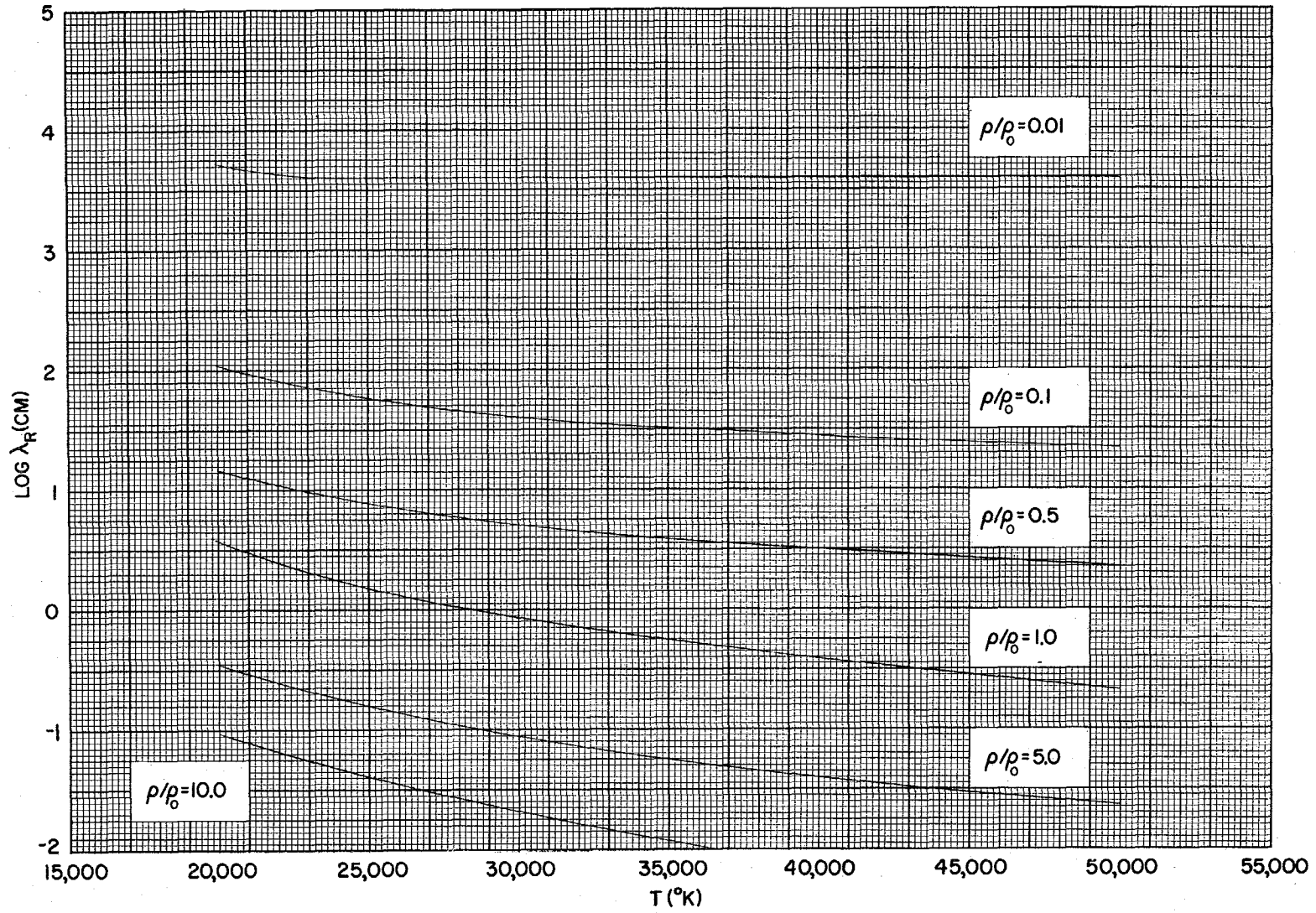
Fig. 3.2 Rosseland mean free path
