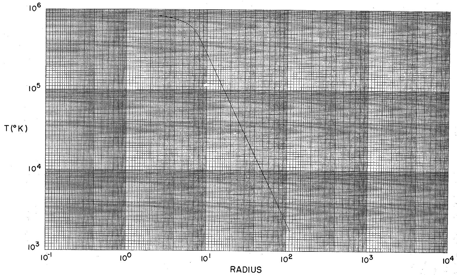
Fig. 3.11 Shock temperature vs shock radius
