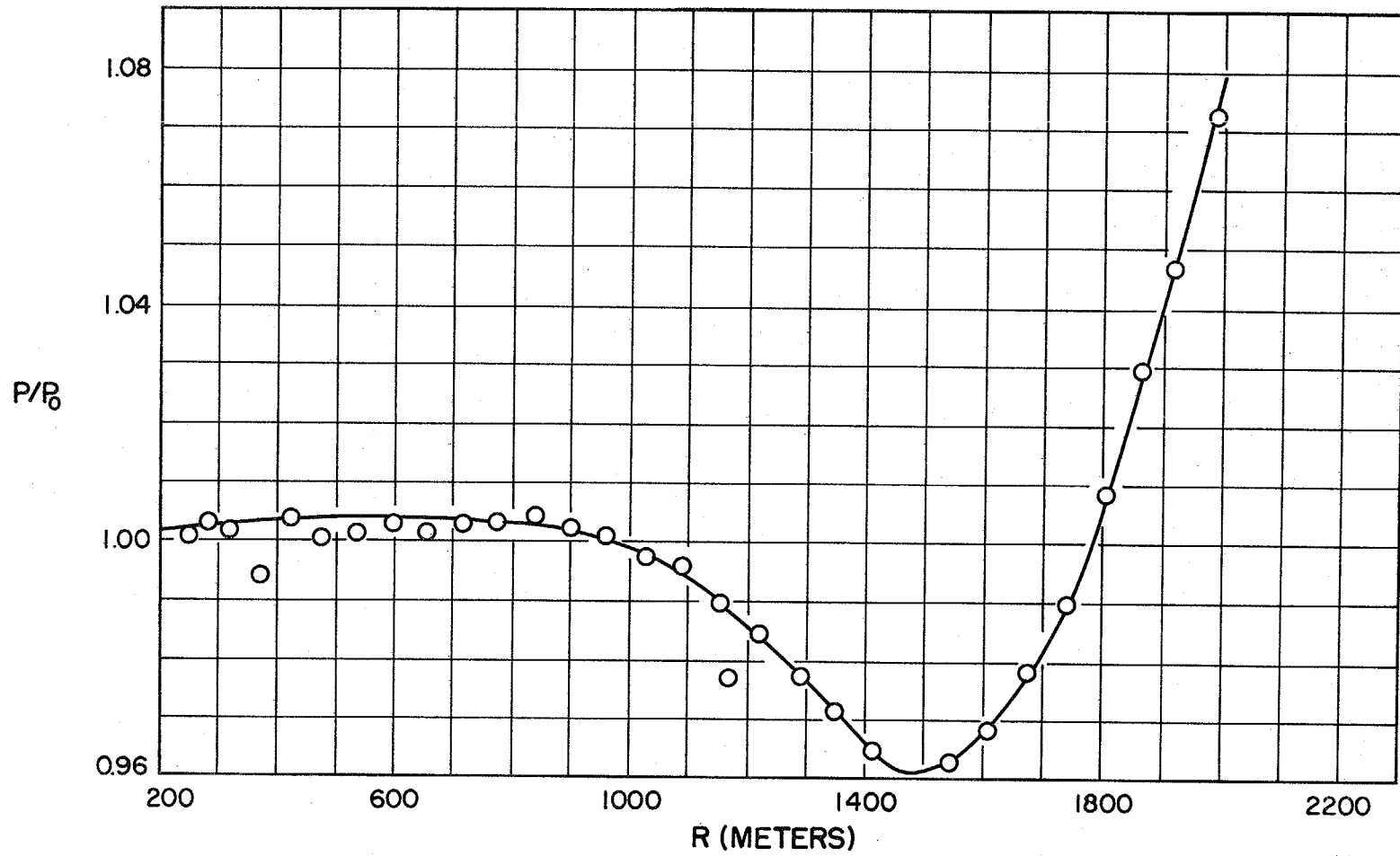
Fig. 6.12 Pressure vs distance at a fixed time
