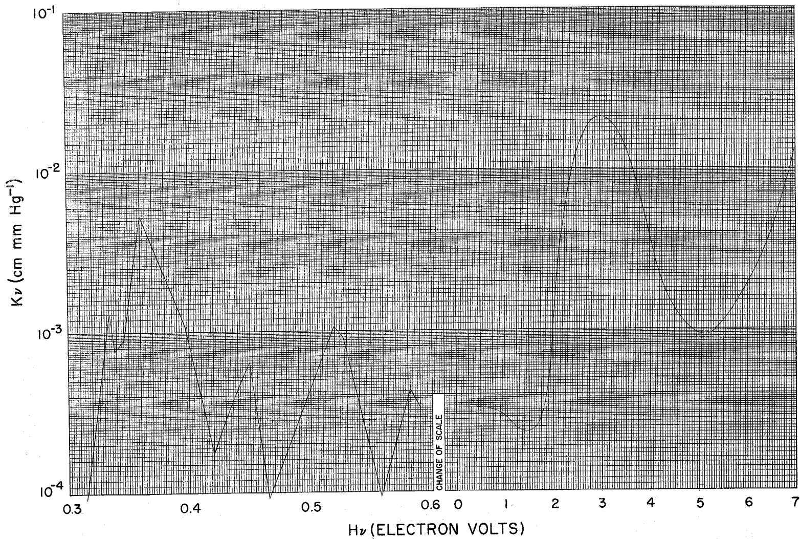
Fig. 3.4 Absorption coefficient of \text{NO}_2 for T \approx 300^\circ\text{K}
