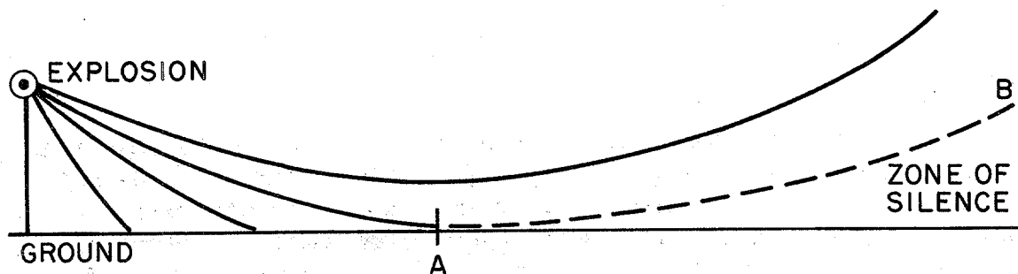
Fig. 1.1 Path of acoustic waves starting from the center "0"
