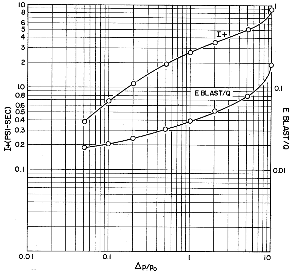
Fig. 6.15 The positive impulse and the energy in the blast. IBM run scaled to 40,000 tons in free air. (Q is the total energy.)
