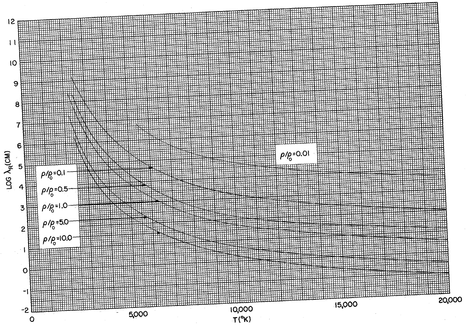
Fig. 3.3 Mean free path for absorption of radiation by \text{O}^- and \text{O}_2^- ; \lambda = 1/\rho\bar{K}
