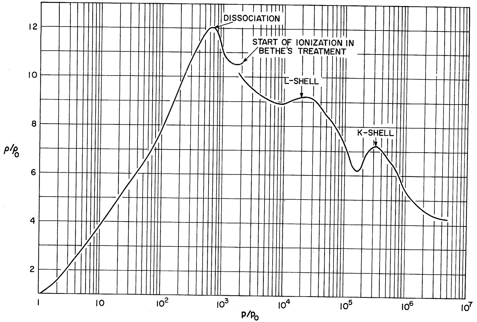
Fig. 7.2 Hugoniot curve; density vs pressure
