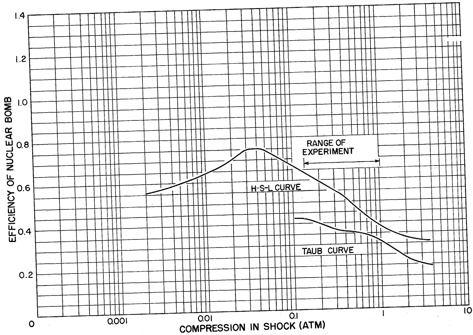
Fig. 6.16 Efficiency of nuclear bomb as compared to an equivalent charge of TNT
