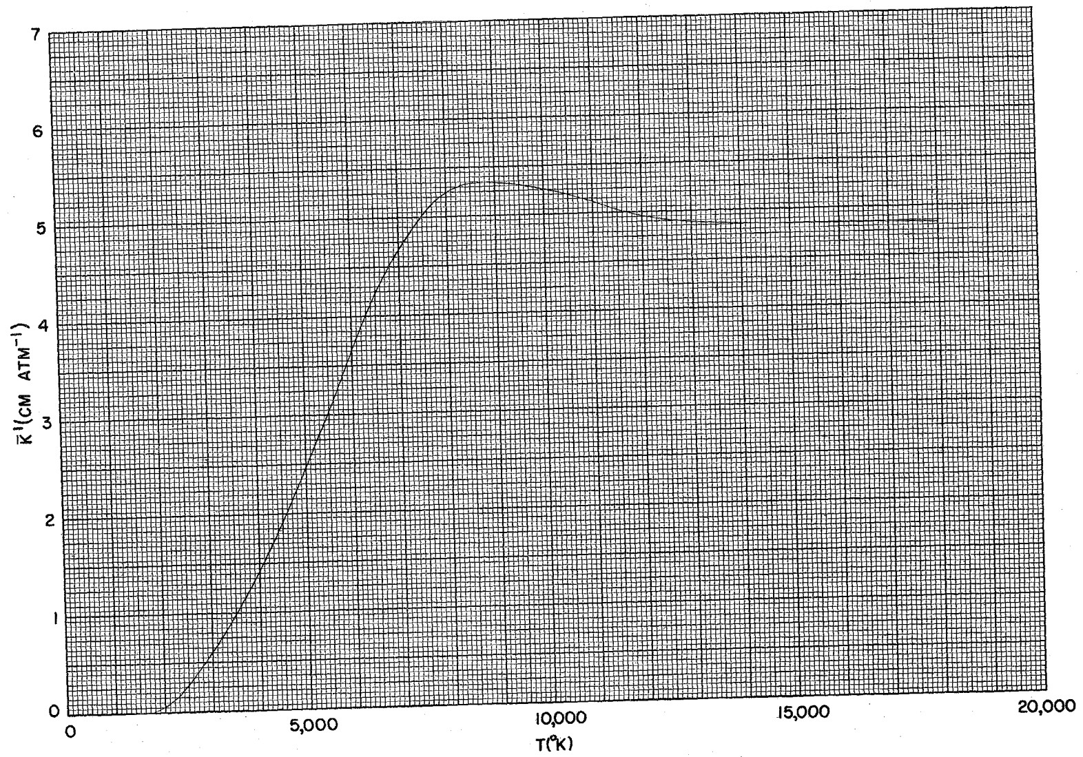
Fig. 3.5 Mean free path of radiation in \text{NO}_2 , \lambda = 1/\bar{K}' P(\text{NO}_2)
