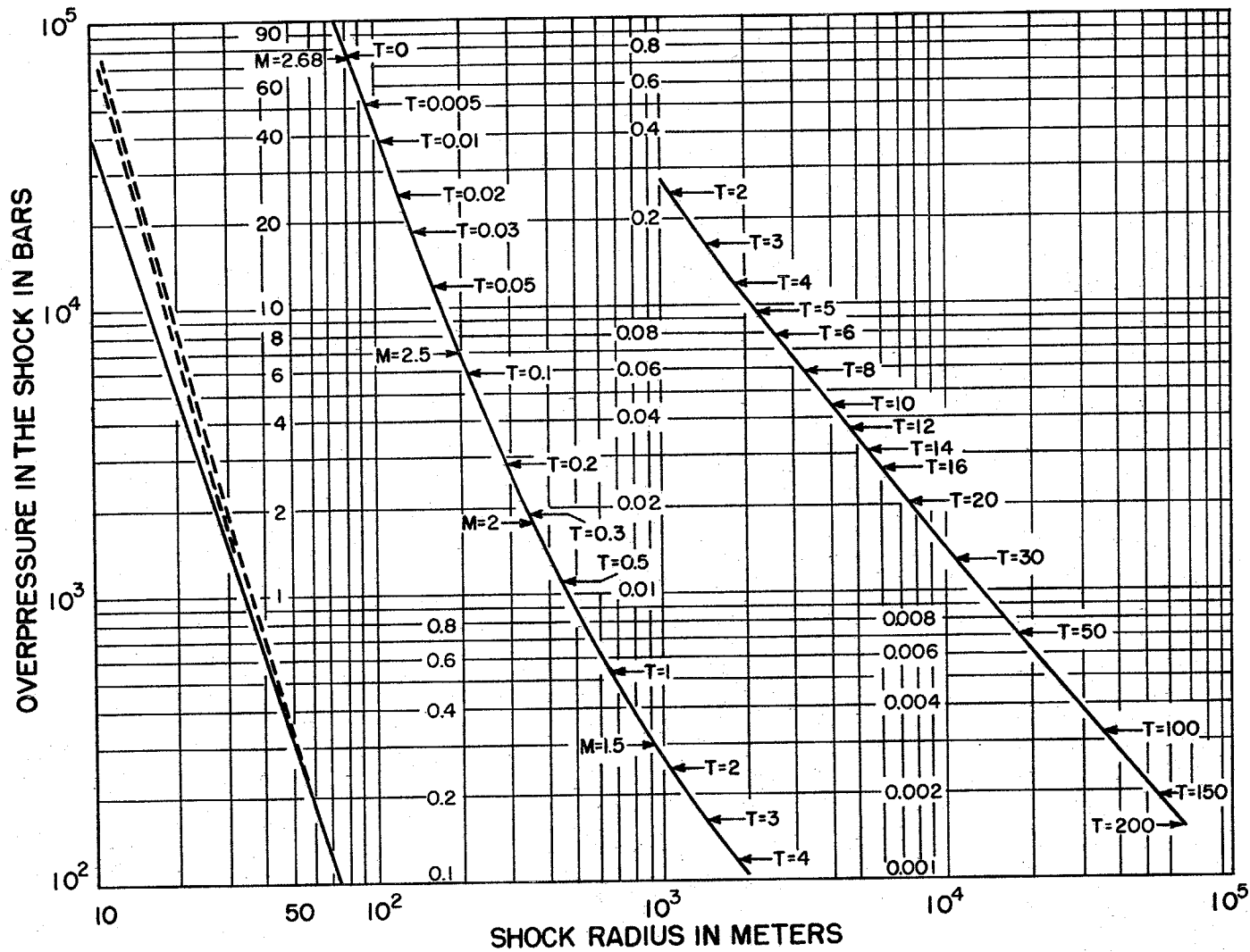
Fig. 6.1 Shock pressure vs distance for nuclear explosion. Time is given in seconds; T = 0 is start of IBM run, 0.012 sec after explosion.
