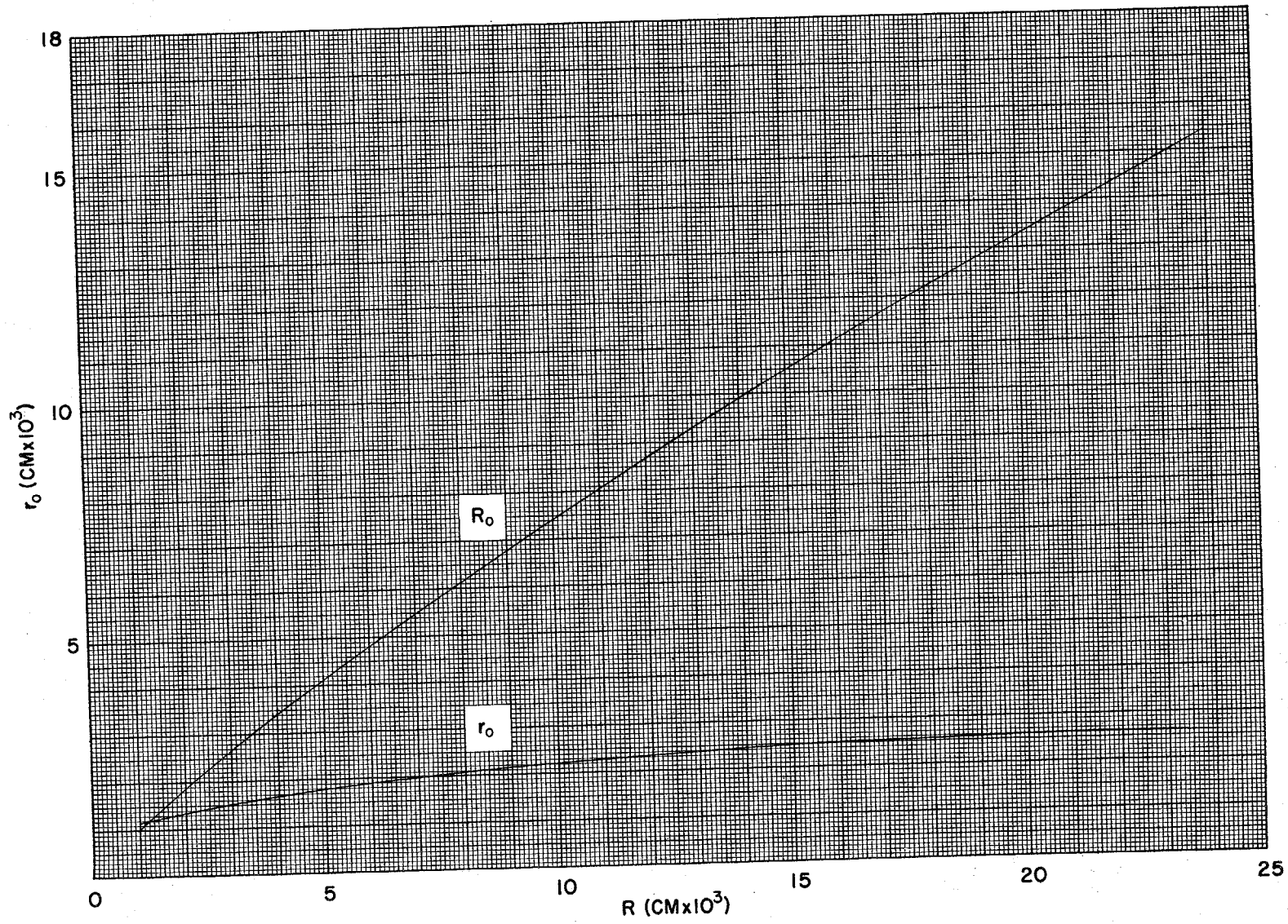
Fig. 3.9 Radius of internal radiation front ( r_0 ) vs shock radius (R)
